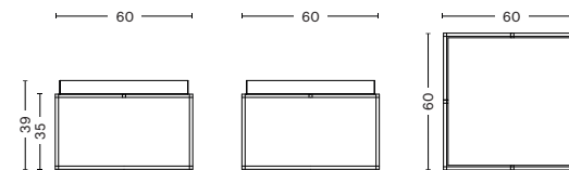
TRAY TABLE COFFEE L60 x W60 x H39 cm
