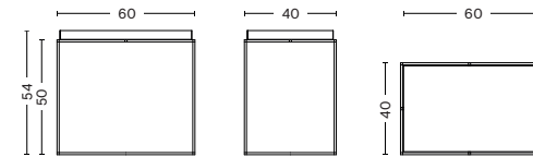
TRAY TABLE L L60 x W40 x H54 cm
