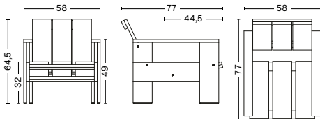
CRATE LOUNGE CHAIR WIDTH 58 CM DEPTH 77 CM HEIGHT 64,5 CM SEAT HEIGHT 32 CM SEAT DEPTH 44,5 CM
